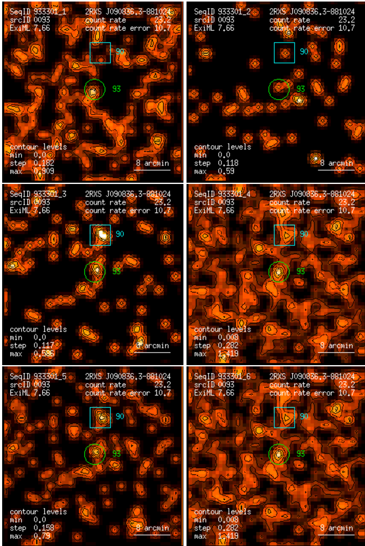
Figure 93: RASS 933301: detection 0093: band rate images, Gaussian filter: (1) PSPC channels 11 – 41, (2) 52 – 90, (3) 91 – 201, (4) 11 – 235, (5) 52 – 201, (6) 11 – 201. Broad band rates in counts/ks. Band rate contour levels in counts/ks/arcmin 2 .
