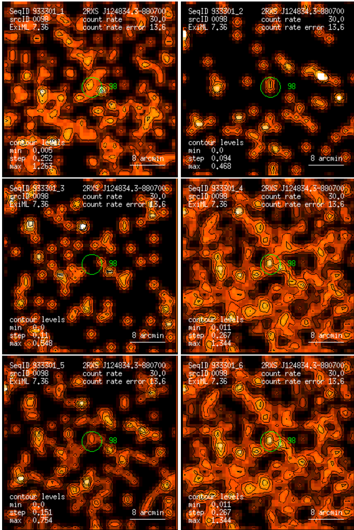
Figure 98: RASS 933301: detection 0098: band rate images, Gaussian filter: (1) PSPC channels 11 – 41, (2) 52 – 90, (3) 91 – 201, (4) 11 – 235, (5) 52 – 201, (6) 11 – 201. Broad band rates in counts/ks. Band rate contour levels in counts/ks/arcmin 2 .
