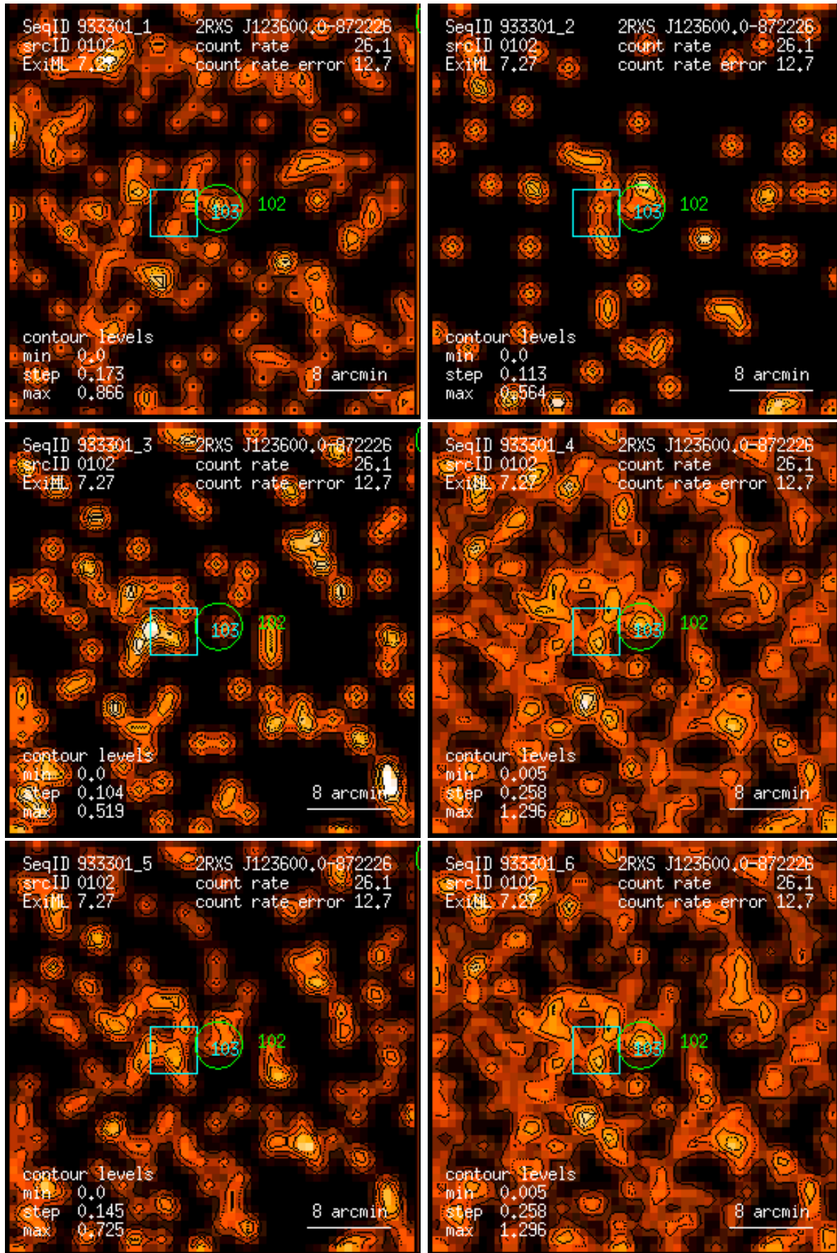
Figure 102: RASS 933301: detection 0102: band rate images, Gaussian filter: (1) PSPC channels 11 – 41, (2) 52 – 90, (3) 91 – 201, (4) 11 – 235, (5) 52 – 201, (6) 11 – 201. Broad band rates in counts/ks. Band rate contour levels in counts/ks/arcmin 2 .
